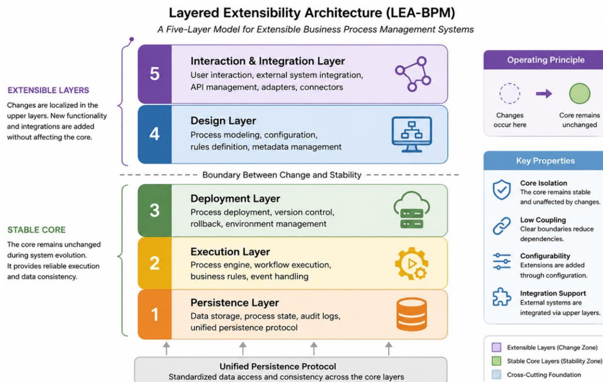
Figure 1. Layered Architecture for BPM System Extensibility (Author's elaboration)
